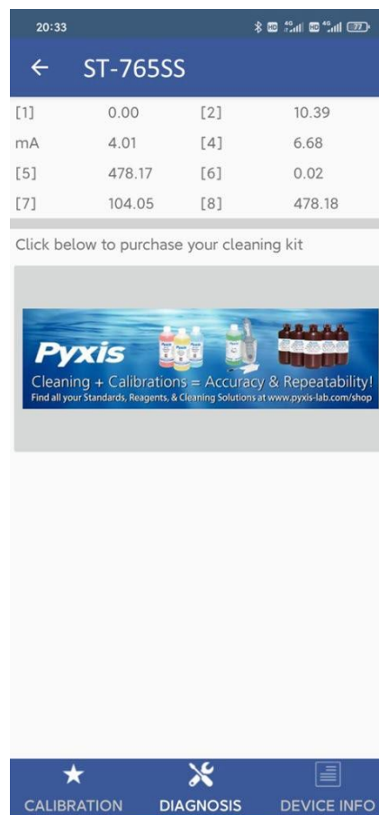
Figure 12 Diagnostic Interface
