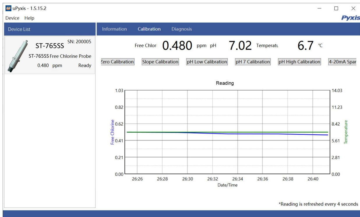
Figure 17. Calibration Page
