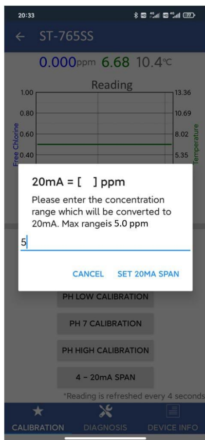
Figure 11 Enter free chlorine concentration to set 4-20mA
