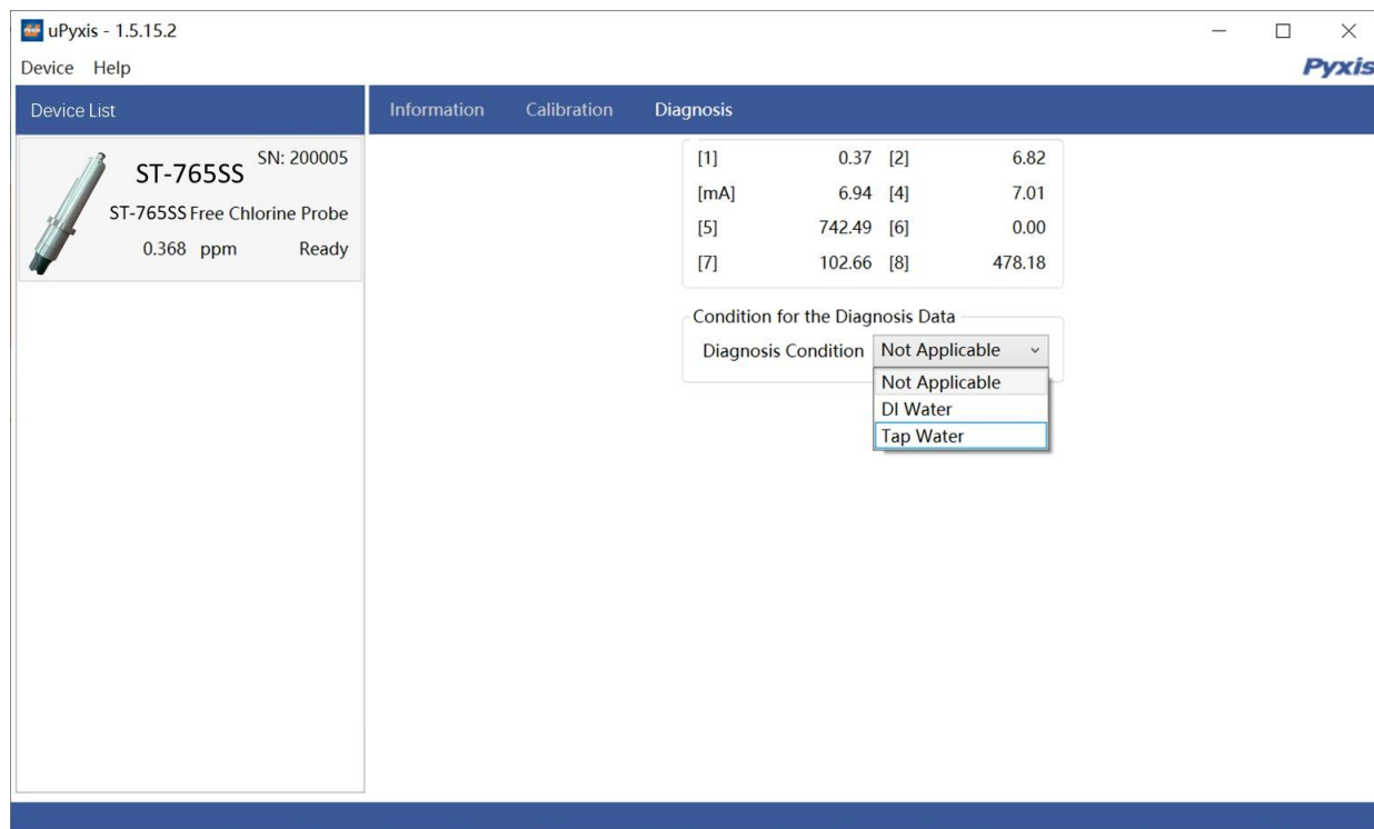
Figure 23 Diagnostic Interface
