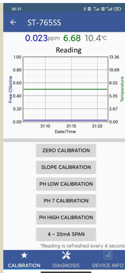
Figure 7. Calibration page
