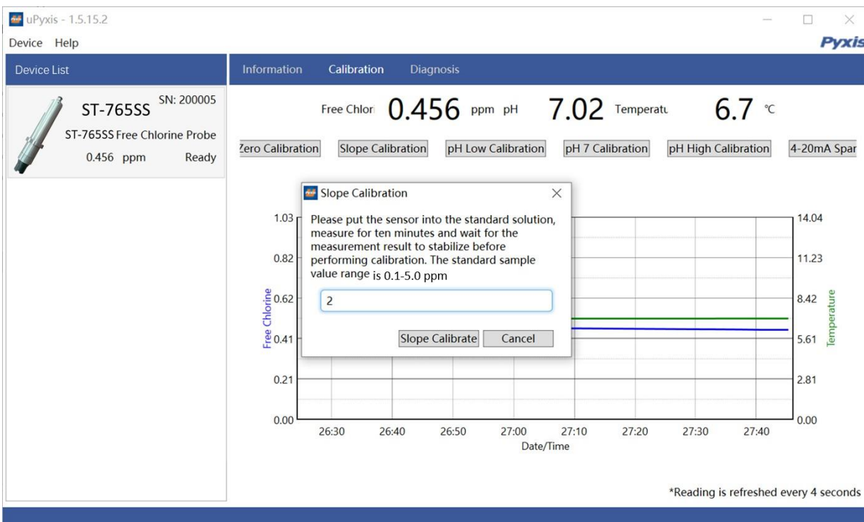
Figure 18 Slope Calibration
