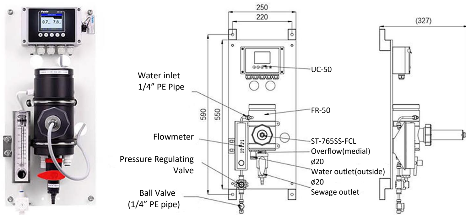
Figure 4 – IK-765SS Series Panel
